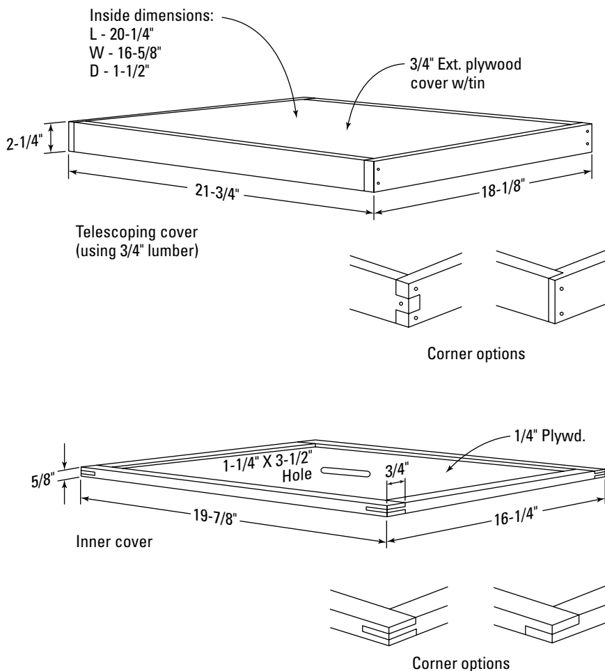
Figure 16-4: These blueprints will serve as a guide if you decide to build your own hive.
