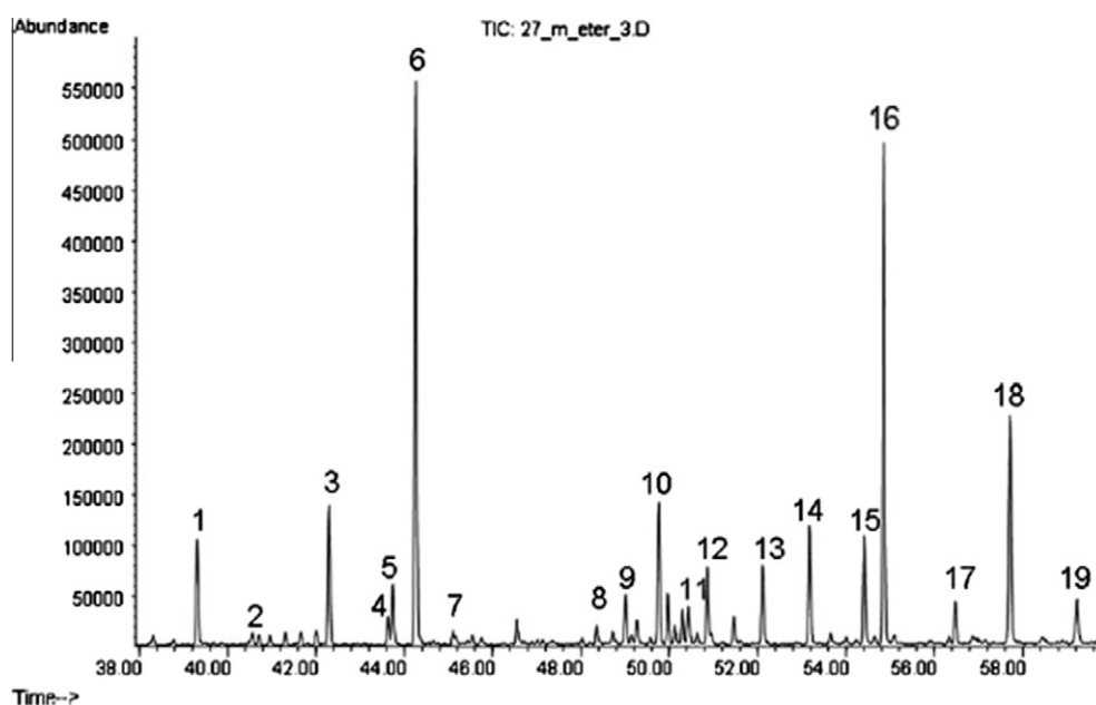
Fig. 5 – Chromatogram of carboxylic acids extracted from honeydew honey (HDH-5). (1) Salicylic acid, (2) 7-hydroxyoctanoic acid, (3) spheryllactic acid, (4) 8-hydroxyoctanoic acid, (5) 4-hydroxybenzoic acid, (6) 4-hydroxybenzeneacetic acid, (7) 3-hydroxydecanoic acid, (8) 2-octene-1,8-dioic acid, (9) 3,4-dihydroxyphenylethanol, (10) homovanillic acid, (11) 10-hydroxydecanoic acid, (12) protocatechuic acid, (13) 10-hydroxy-2-decenoic acid (10-HDA), (14) sebaccic acid, (15) p-coumaric acid, (16) 2-decene-1,10-dioic acid, (17) 3,10-dihydroxydecanoic acid, (18) hexadecanoic acid, (19) ferulic acid.
